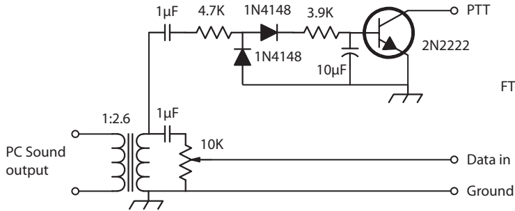
FT-817 sound card interface Thanks to VK2ZAY
